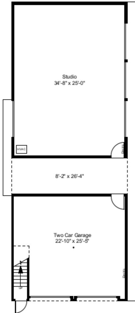
First Floor Plan Ceiling Height = 8'-3"
